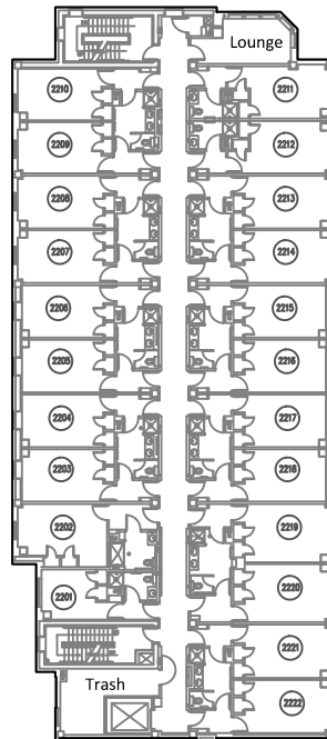
KOENIG SECOND FLOOR
